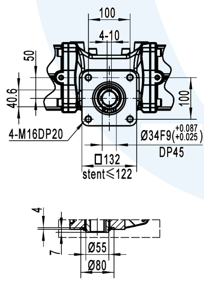
Connection size of bottom valve
