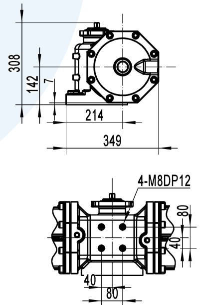
Side connection size
