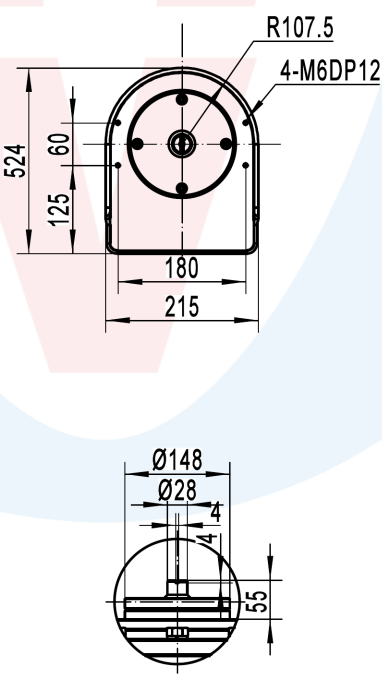
Top connection size
