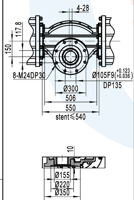
Connection size of bottom valve
