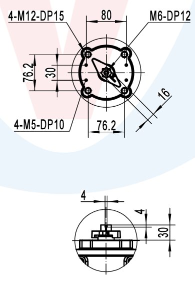
Top connection size
