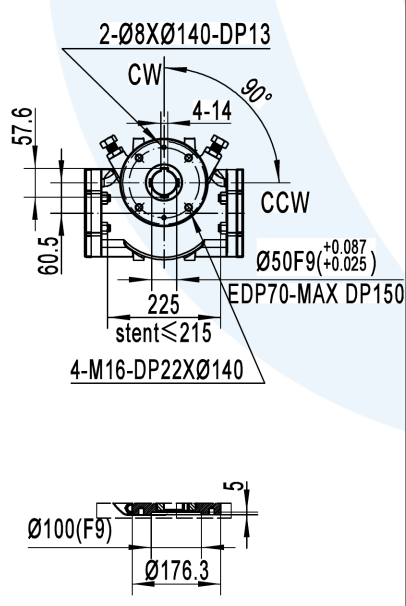
Connection size of bottom valve
