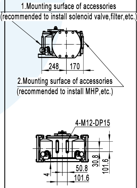
Side connection size
