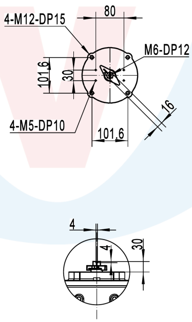
Top connection size
